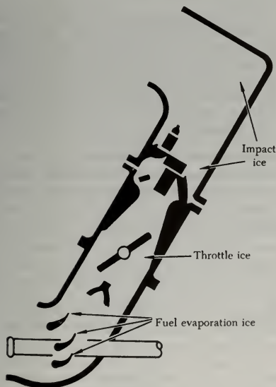
FIGURE 2-2. Types of induction system ice.
